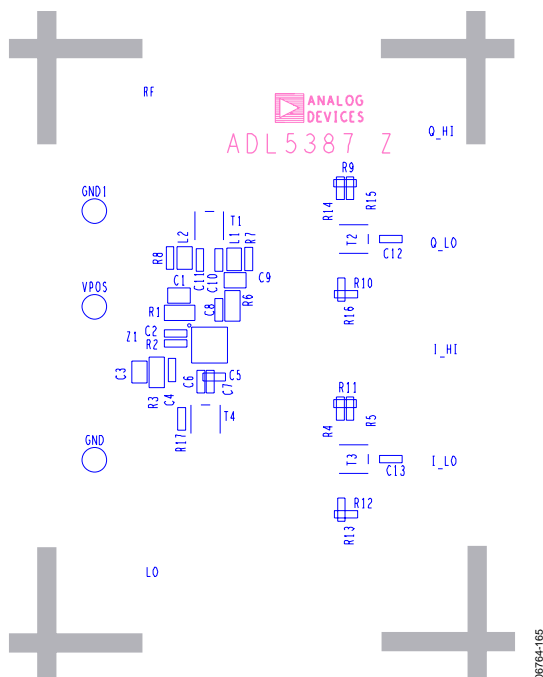
Figure 69. Evaluation Board Top Layer Silkscreen
