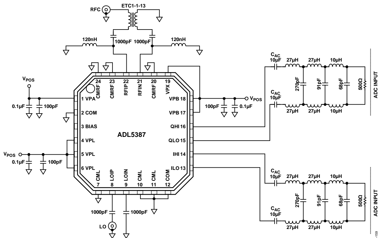
Figure 63. Sixth Order Low-Pass Butterworth Baseband Filter Schematic
