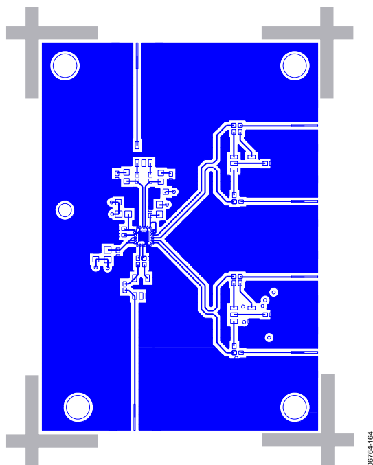
Figure 68. Evaluation Board Top Layer
