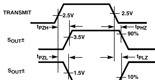
FIGURE 3B. MEASUREMENT POINTS
