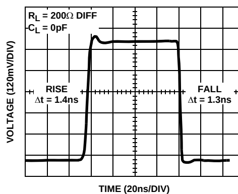
FIGURE 16. DIFFERENTIAL SMALL SIGNAL TRANSIENT RESPONSE
