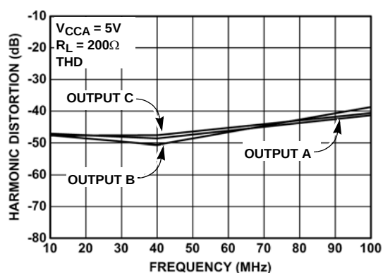
FIGURE 12. TOTAL HARMONIC DISTORTION
