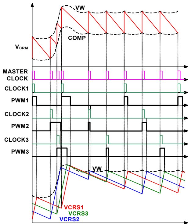
FIGURE 10. R3™ MODULATOR OPERATION PRINCIPLES IN LOAD INSERTION RESPONSE
