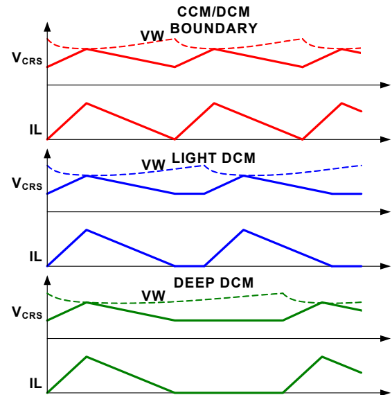
FIGURE 12. PERIOD STRETCHING
