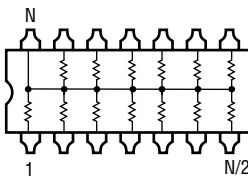
-1 Circuit - Bussed Resistors
