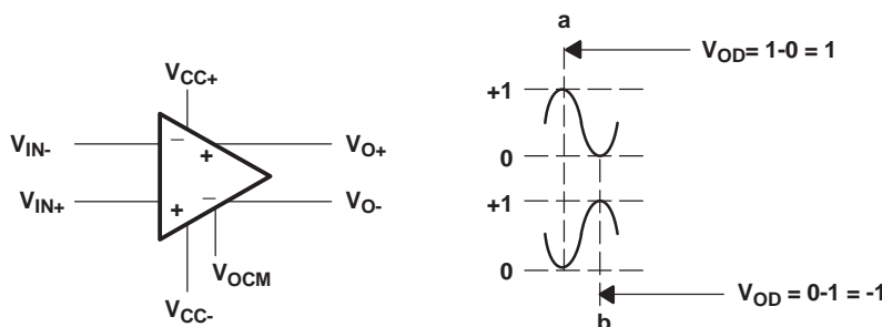
Figure 40. Fully Differential Amplifier With Two 1- V_{PP} Signals
