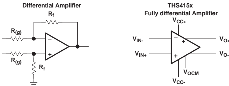
Figure 36. Differential Amplifier Versus a Fully Differential Amplifier
