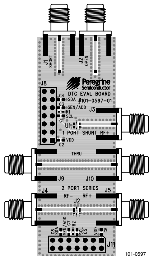
Figure 21. Evaluation Board Layout
