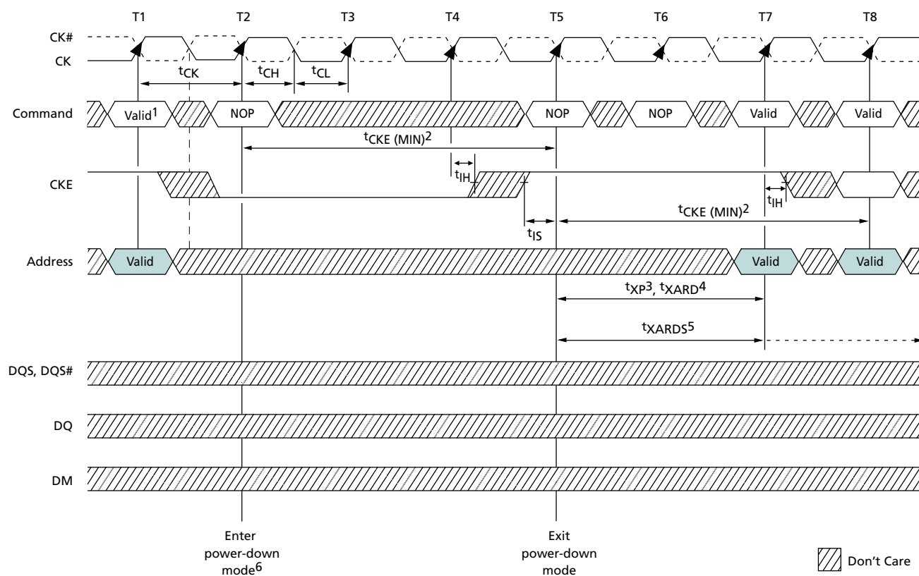
Figure 69: Power-Down
