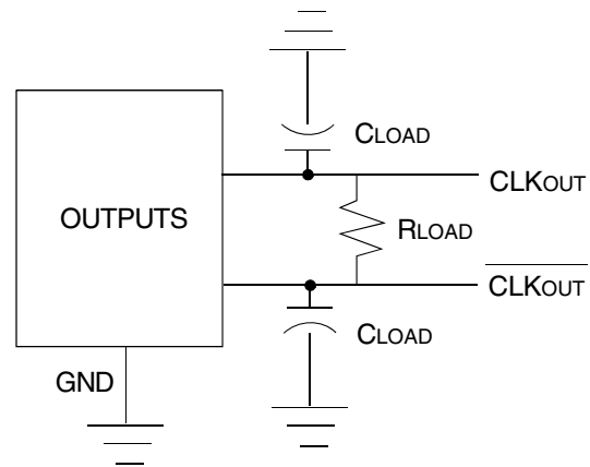
LVDS: - 100 \Omega between differential outputs with 5pF
