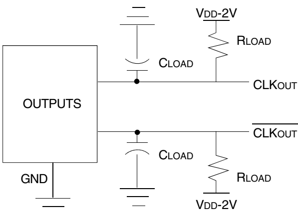
LVPECL: - 50 \Omega to V_{DD}-2V for each output with 5pF
