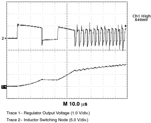
Figure 12. Demonstration Board Enable Startup Waveforms
