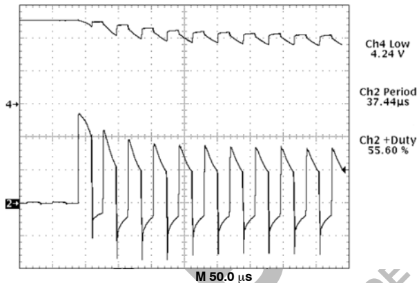
Figure 18. Demonstration Board Hiccup Mode Short Circuit Protection. Gate Pulses are Delivered While the Soft Start Capacitor Charges, and Cease During Discharge
