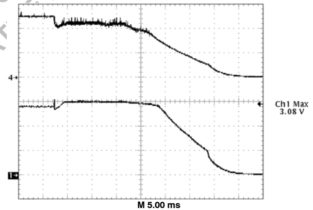
Figure 20. OVP Response to an Input-to-Output Short Circuit by Immediately Providing 0% Duty Cycle, Crow-Barring the Input Voltage to Ground
