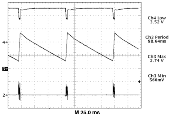
Figure 18. Demonstration Board Hiccup Mode Short Circuit Protection. Gate Pulses are Delivered While the Soft Start Capacitor Charges, and Cease During Discharge
