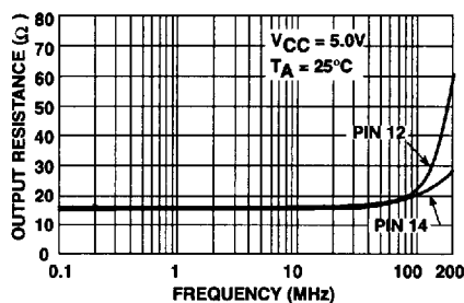
Output Resistance vs Frequency
