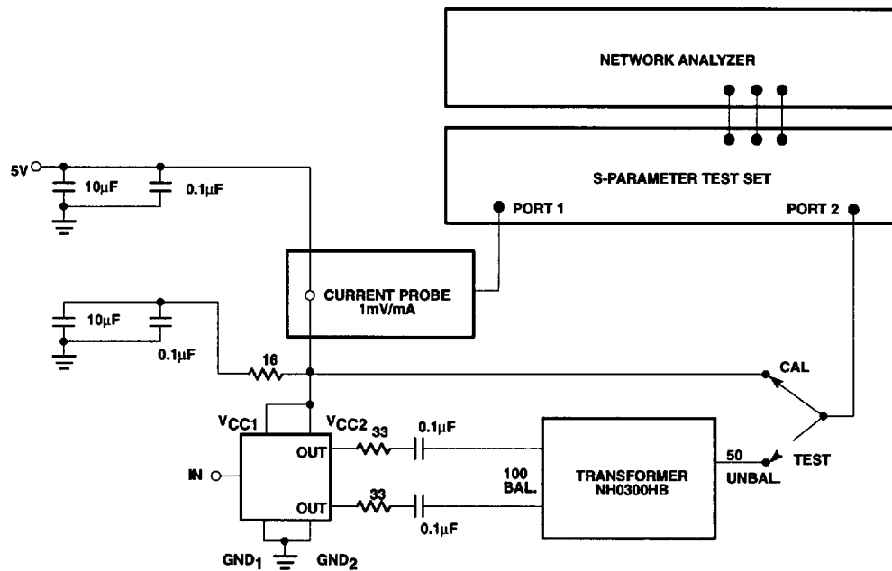
Test Circuit 3
