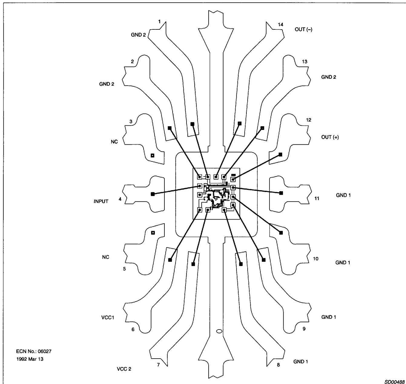
Figure 5. NE5210 Bonding Diagram
