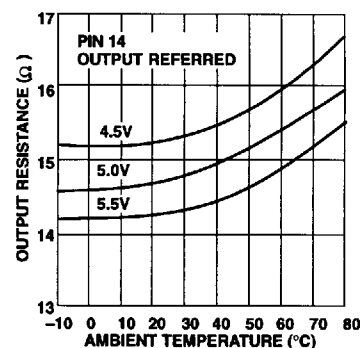
NE5210 Output Resistance vs Temperature
