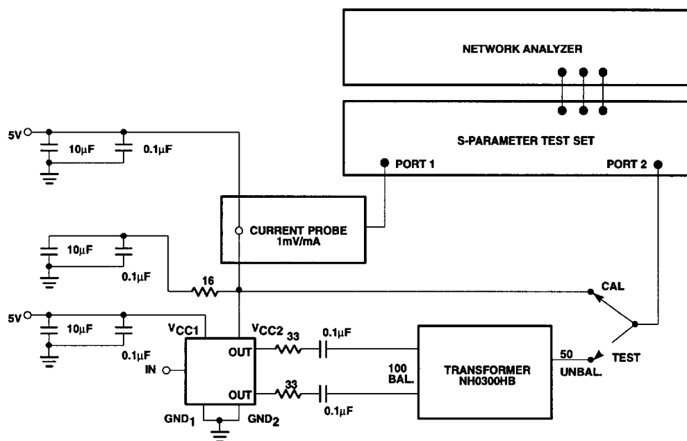
Test Circuit 5
