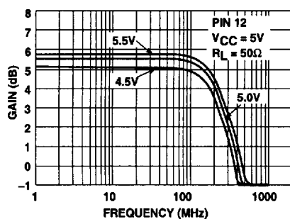
Gain vs Frequency
