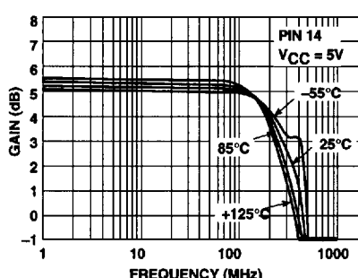
Gain vs Frequency
