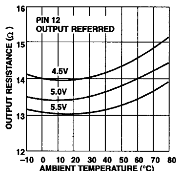
NE5210 Output Resistance vs Temperature
