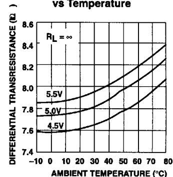
NE5210 Differential Transresistance vs Temperature
