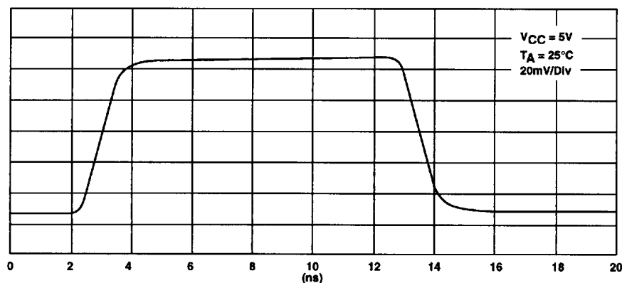
Output Step Response
