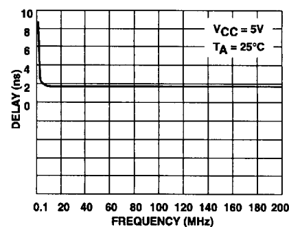
Group Delay
