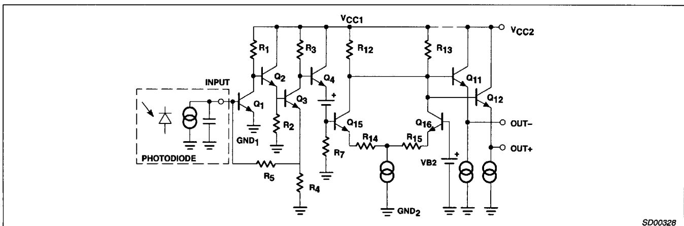
Figure 2. Transimpedance Amplifier
