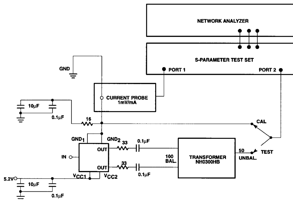
Test Circuit 6
