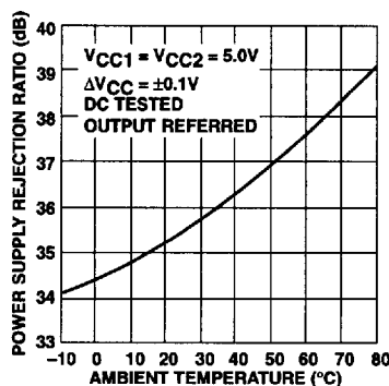
NE5210 Power Supply Rejection Ratio vs Temperature
