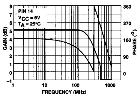
Gain and Phase Shift vs Frequency
