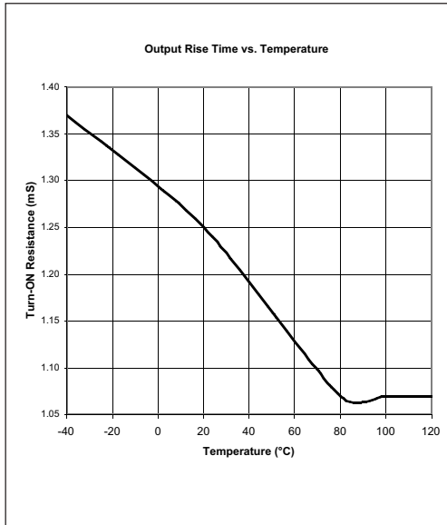
Figure 9. Output Rise Time vs. Temperature
