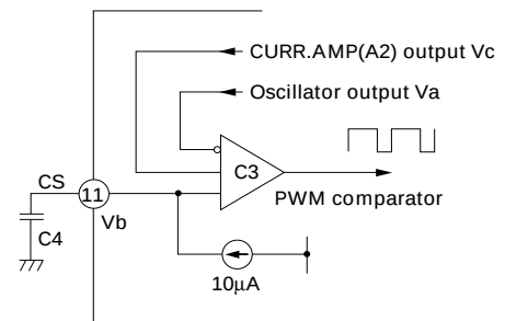
Fig. 5 PWM comparator
