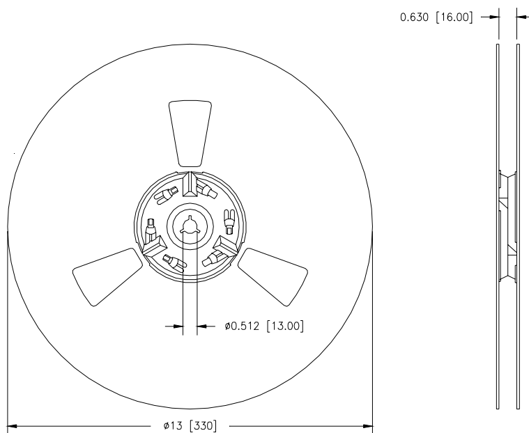
Figure 16: Reel Dimensions
