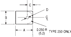
TO-220
