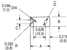
TO-66 (RECTANGLE)
