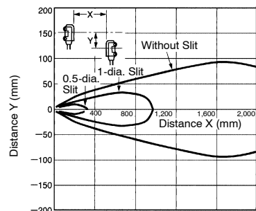
E3T-FT1□ with Slit (Through-Beam)
