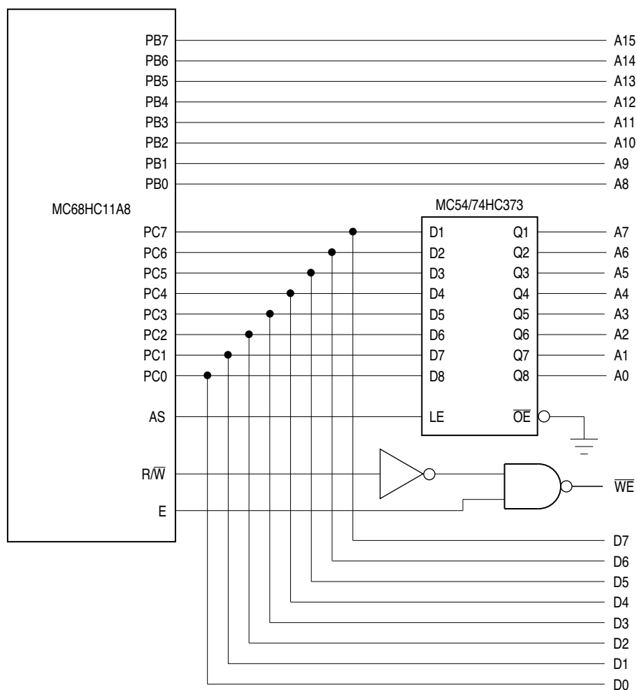
Figure 4 Address/Data Demultiplexing
