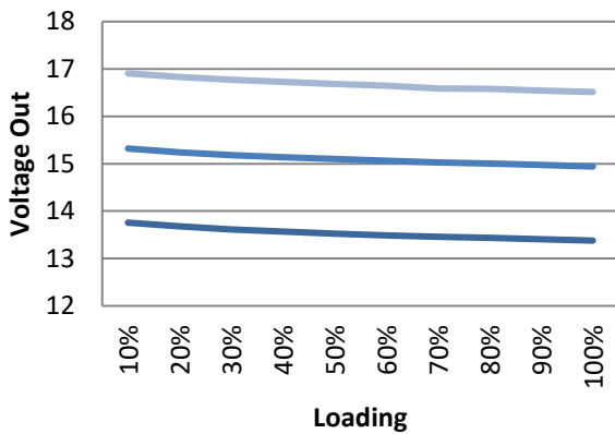
AM1/4S-0515SZ Load vs. Vout
