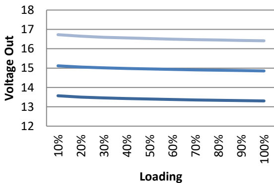
AM1/4S-1215SZ Load vs. Vout
