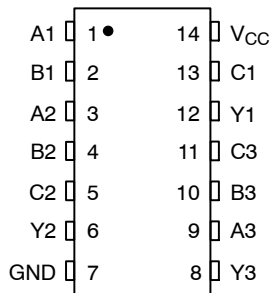
Figure 2. Pinout Diagram
