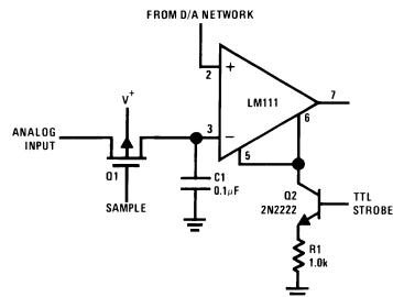
Strobing off Both Input and Output Stages (Note 2)
