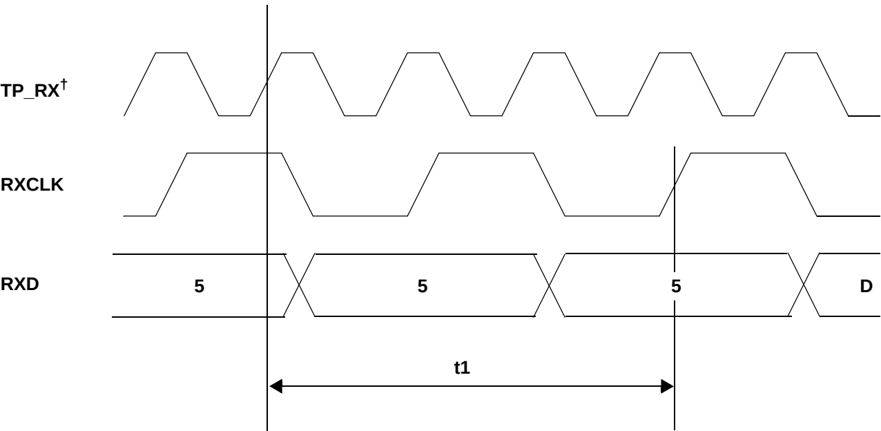
10M MII Receive Latency Timing Diagram
