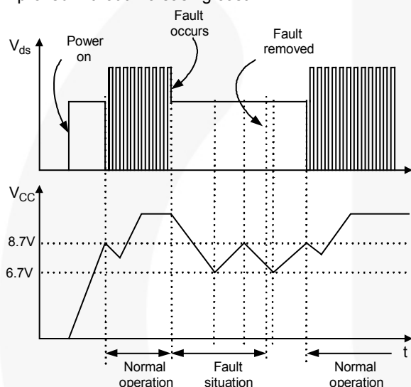
Figure 16. Auto Restart Protection Waveforms
