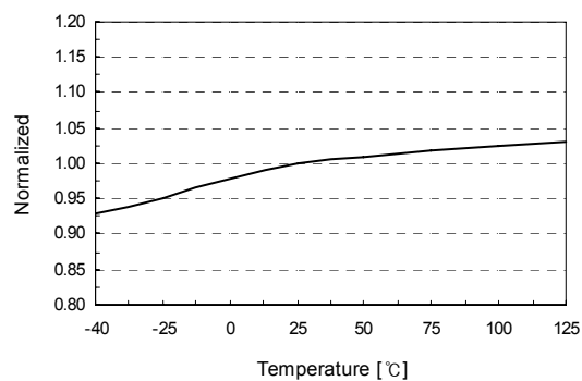
Figure 11. Shutdown Delay Current ( I_{DELAY} ) vs. T_A
