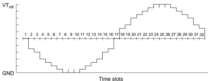
Figure 75 Waveform of Tone Output
