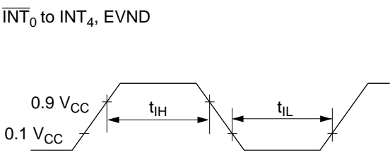
Figure 92 Interrupt Timing
