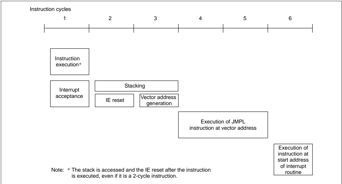
Figure 10 Interrupt Sequence
