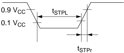
Figure 94 STOPC Timing
