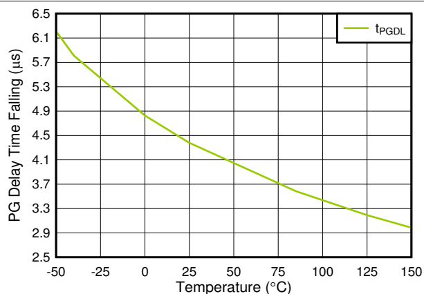
Figure 6-26. t_{PGDL} vs Temperature
