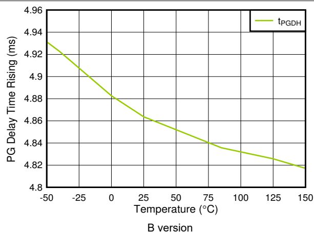
Figure 6-25. t_{PGDR} vs Temperature (For TPS746B Only)
