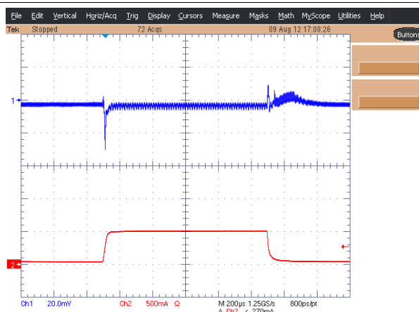
Figure 74. DCDCx Load Transient Response, 1.5 V_{OUT} , 50-500-50 mA Load
