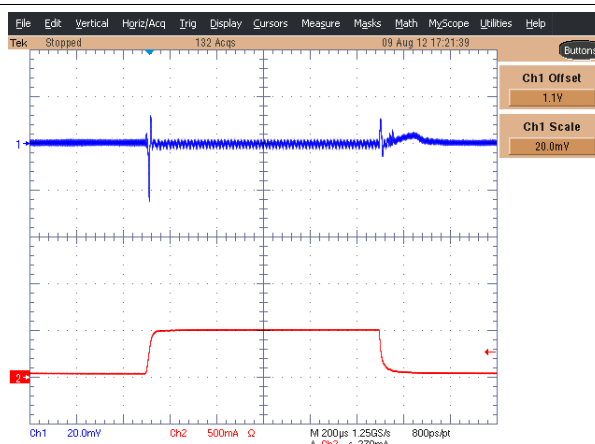
Figure 72. DCDCx Load Transient Response, 1.1 V_{OUT} , 50-500-50 mA Load
