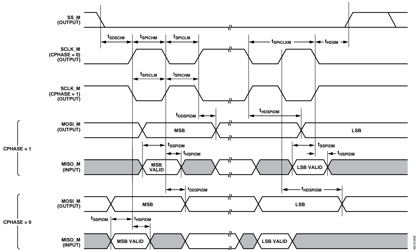
Figure 9. SPI Master Port Timing Specifications
