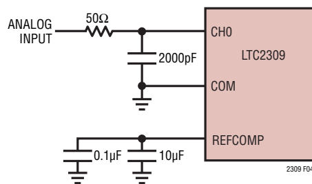
Figure 4a. Optional RC Input Filtering for Single-Ended Input
