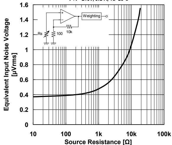
Voltage Noise vs. Source Resistance
