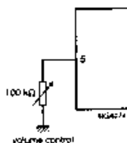
Fig. 7 Application using a potentiometer for volume control; G_v = 30 dB.
