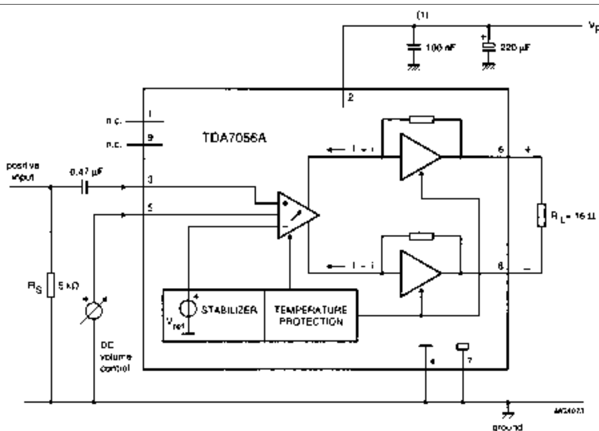
Fig. 6 Test and application diagram.
