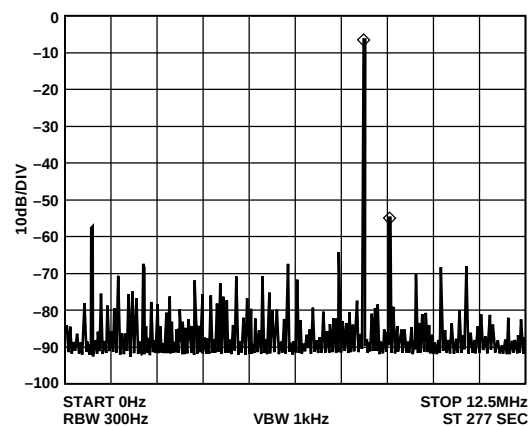
Figure 19. f_{MCLK} = 25 MHz, f_{OUT} = 8.1 MHz, Frequency Word = 52F1A9FC
