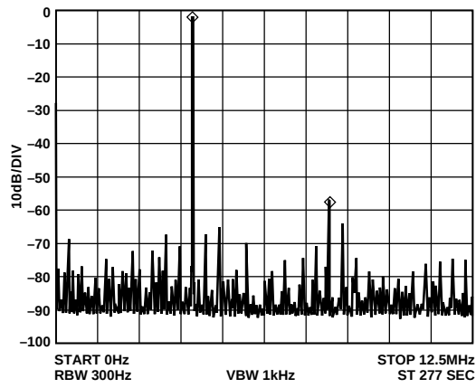
Figure 15. f_{MCLK} = 25 MHz, f_{OUT} = 4.1 MHz, Frequency Word = 29FBE76D
