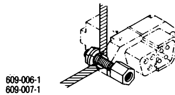
Application for 50 position "D" connectors
