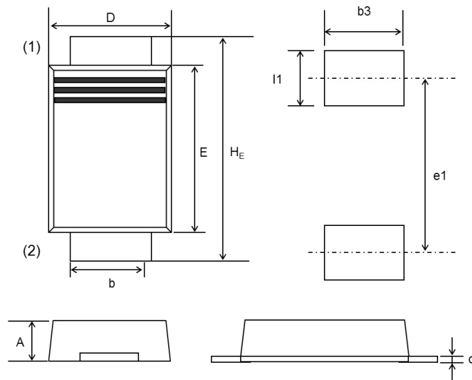
SOD-128, (PMD™)
