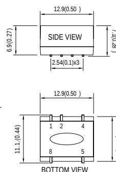
▲ SBTN01 0.50" x 0.43" x 0.28"
