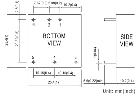
▲ DKMW20 1" x 1" x 0.40"
