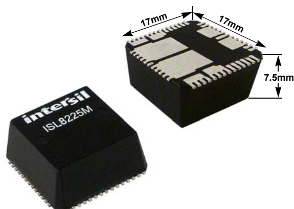
FIGURE 2. SMALL FOOTPRINT WITH HIGH POWER DENSITY
