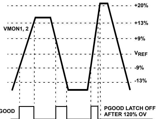
FIGURE 32. POWER-GOOD THRESHOLD WINDOW
