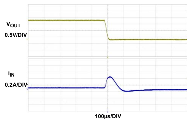
FIGURE 16. SHORT CIRCUIT AT 0A
