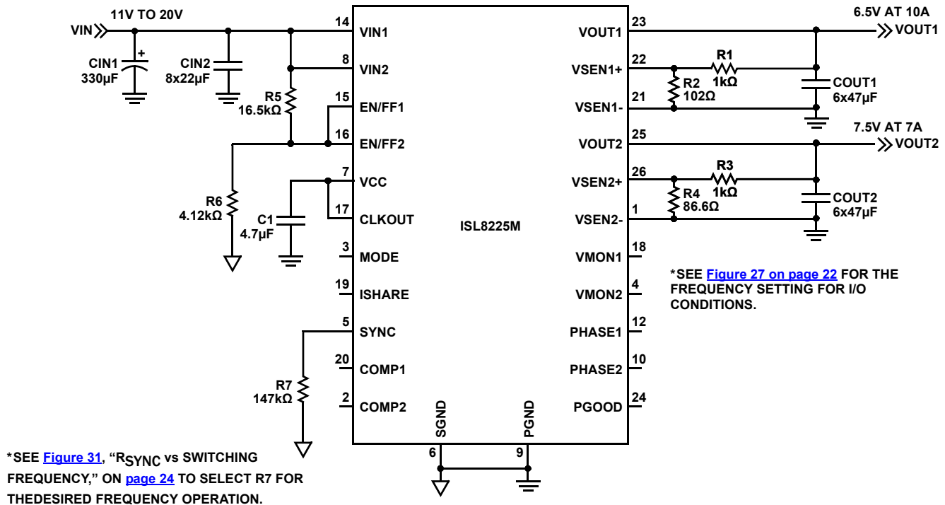
FIGURE 22. HIGH OUTPUT VOLTAGE APPLICATION WITH THE FREQUENCY SET AT 750kHz
