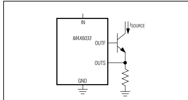
Figure 1. Precision Current Source
