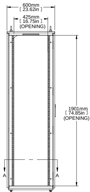
L.S. VIEW
