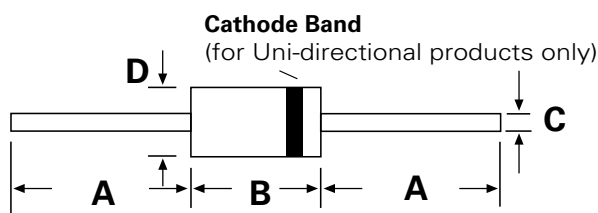
DO-204AC (DO-15)
