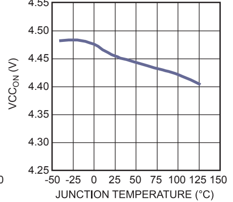
VCC Regulator On Threshold vs. Junction Temperature
