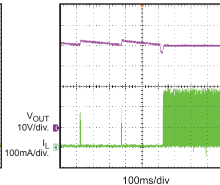
OVP Recovery
