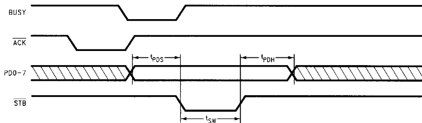
FIGURE 10-16. Typical Parallel Port Data Exchange
