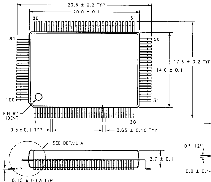
Plastic Quad Flatpak, (EIAJ) (PQFP) Order Number PC87334VLJ NS Package Number VLJ100A
