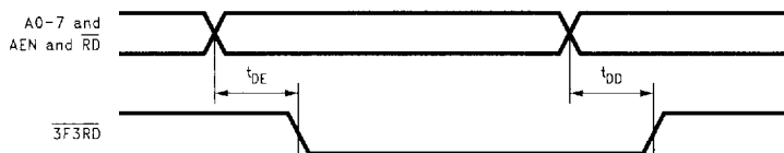
FIGURE 10-20. 3F3 Read Timing
