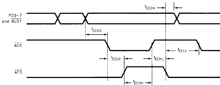
FIGURE 10-19. ECP Parallel Port Backward Timing Diagram
