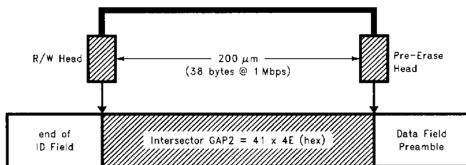
FIGURE 5-3. Perpendicular Recording Drive R/W Head and Pre-Erase Head
