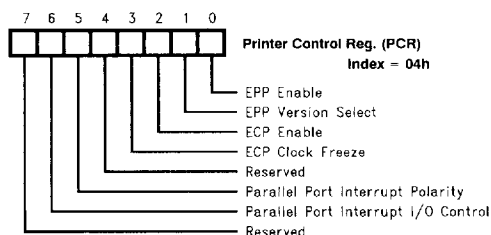
FIGURE 2-1. PC87334VLJ/PC87334VJG Configuration Registers
