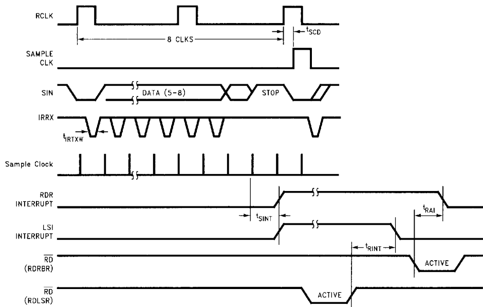
FIGURE 10-6a. Receiver Timing
