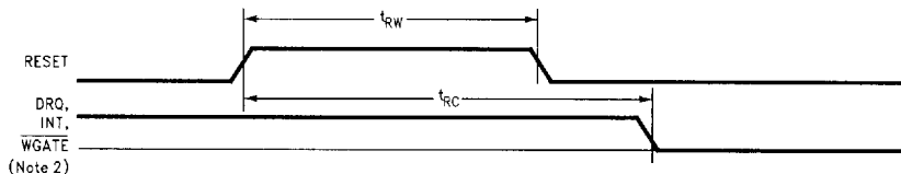
FIGURE 10-9. Reset Timing
