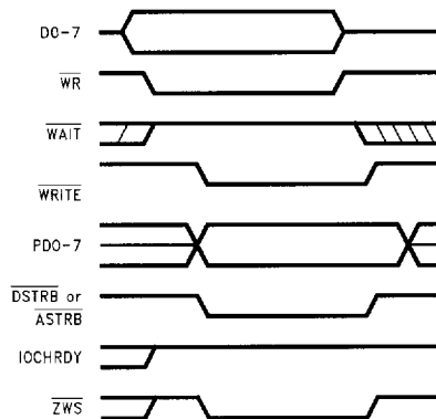
FIGURE 7-3. EPP Write with ZWS
