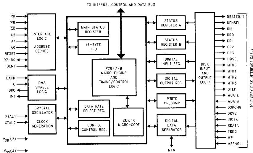
FIGURE 3-1. FDC Functional Block Diagram
