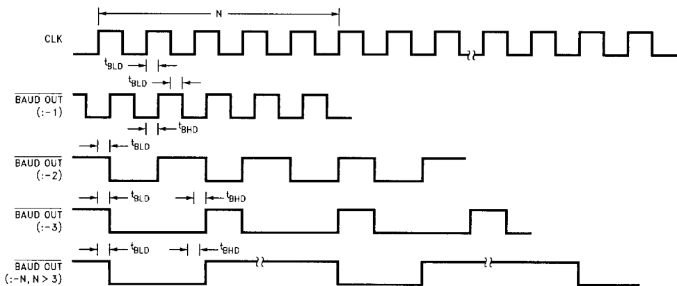
FIGURE 10-4. Baud Out Timing
