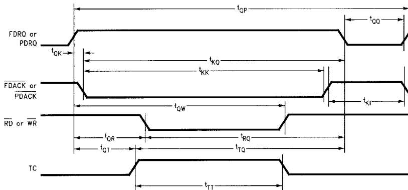
FIGURE 10-8. DMA Timing
