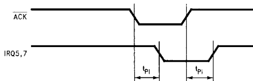
FIGURE 10-14. Compatible Mode Parallel Port Interrupt Timing
