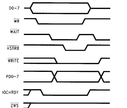
FIGURE 7-4. EPP 1.9 Address Write
