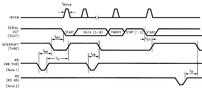
FIGURE 10-5. Transmitter Timing
