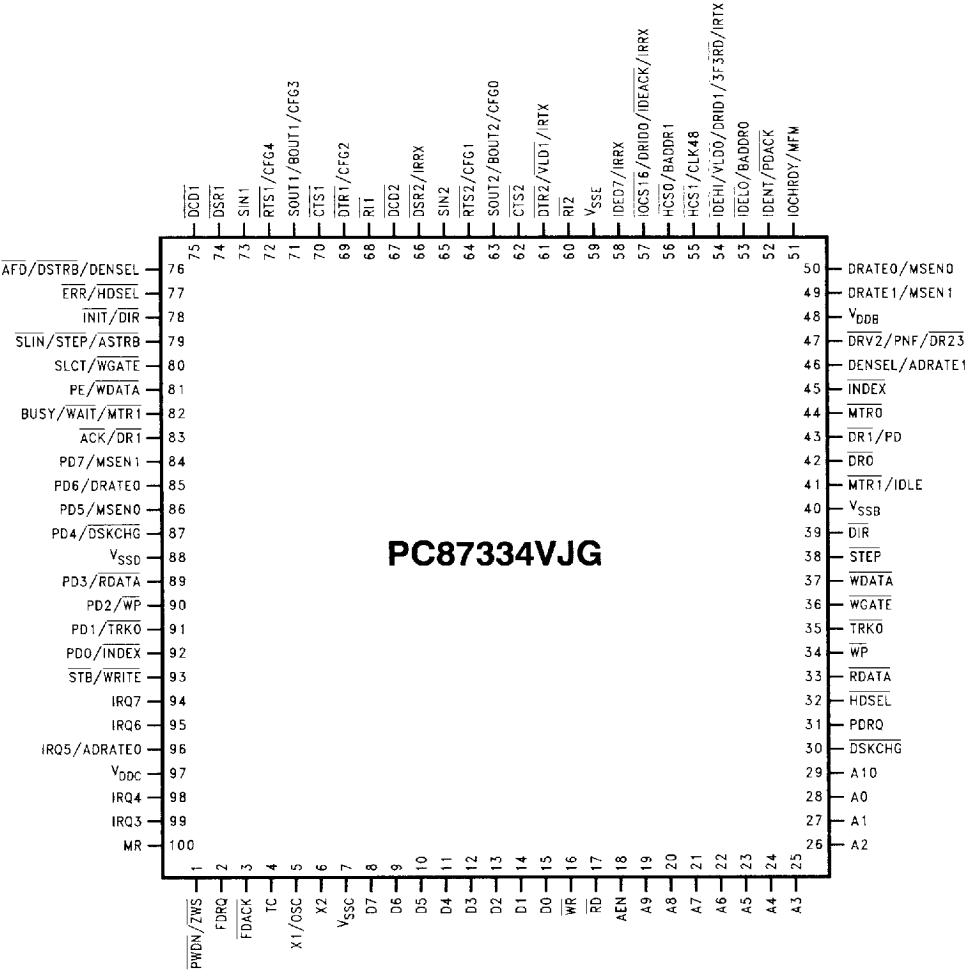
Thin Quad Flatpak (TQFP)
