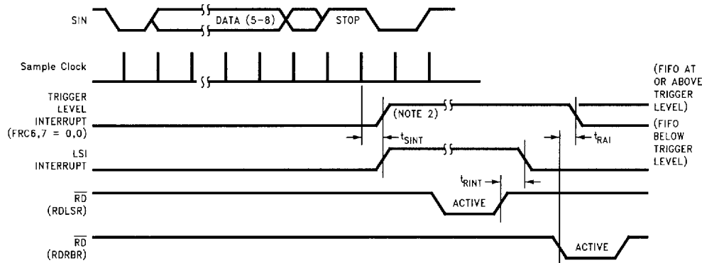
FIGURE 10-6a. Receiver Timing
