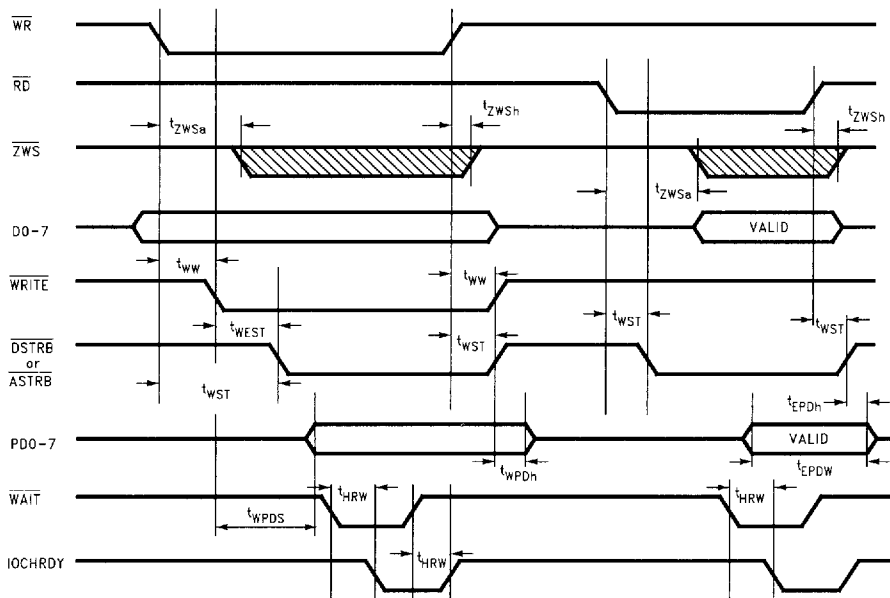
FIGURE 10-17. Enhanced Parallel Port Timing
