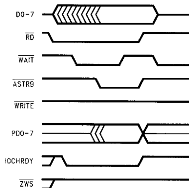
FIGURE 7-5. EPP 1.9 Address Read
