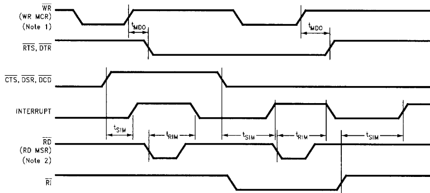
FIGURE 10-7. MODEM Control Timing
