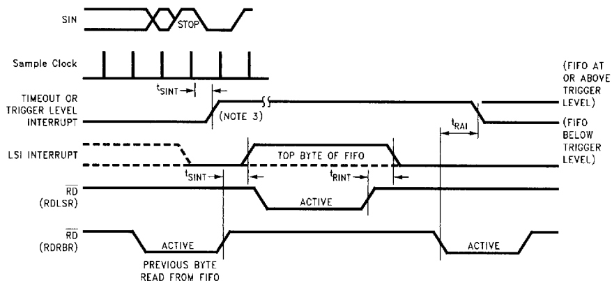
FIGURE 10-6c. Timeout Receiver Timing
