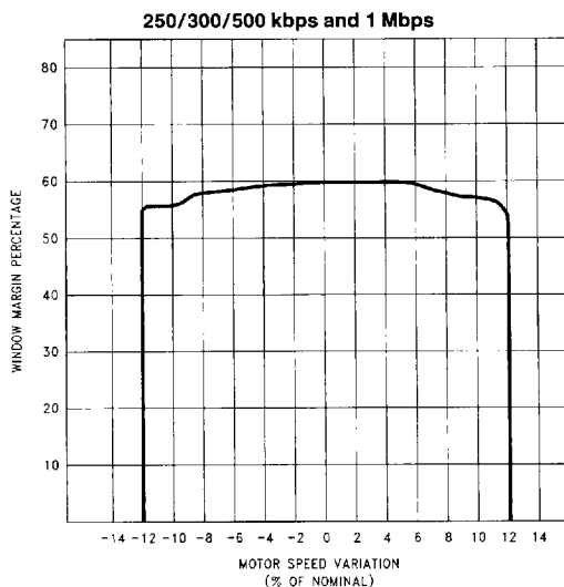
FIGURE 5-1. PC87334 Dynamic Window Margin Performance (Typical Performance at V_{DD} = 5.0V , 25^{\circ}C )
