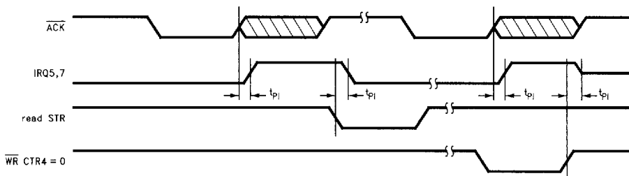
FIGURE 10-15. Extended Mode Parallel Port Interrupt Timing
