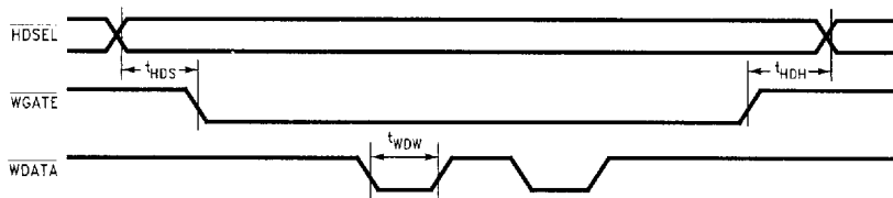
FIGURE 10-10. Write Data Timing
