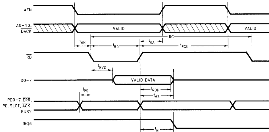
FIGURE 10-2. Microprocessor Read Timing
