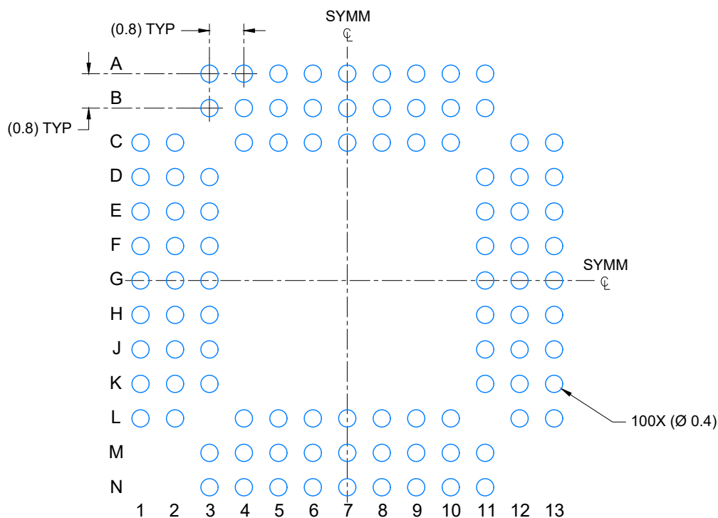
LAND PATTERN EXAMPLE
