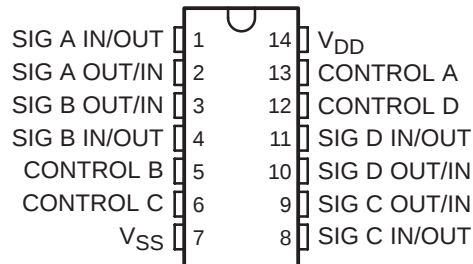
E, F, M, NS, OR PW PACKAGE
