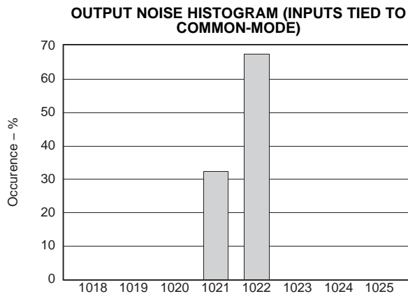
Output Code Figure 26.
