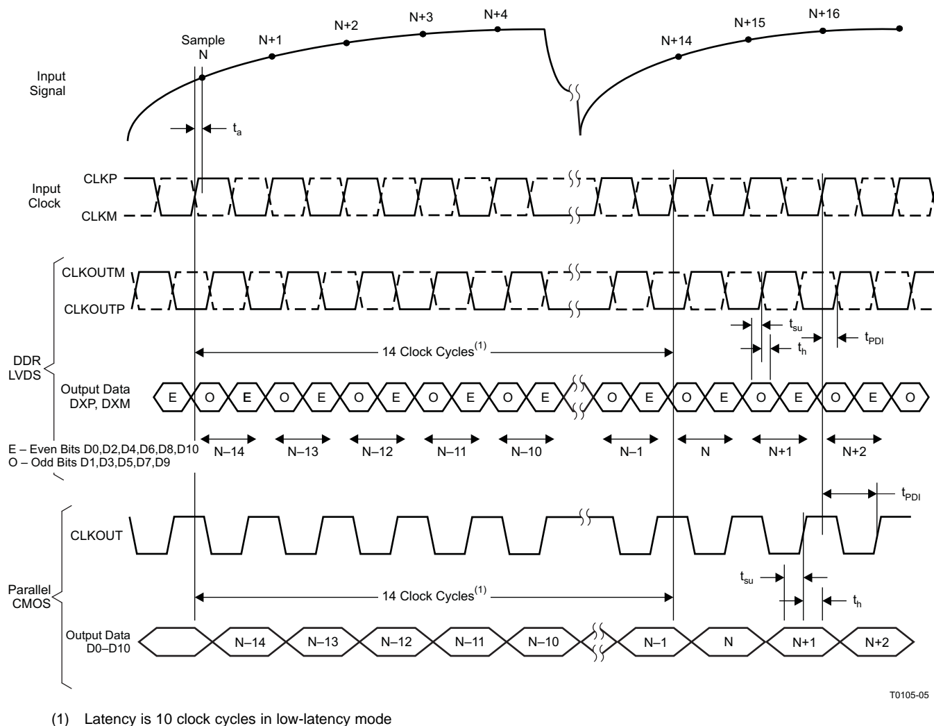
Figure 2. Latency Diagram
