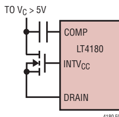
Figure 6. Cascoded DRAIN Pin for Isolated Supplies
