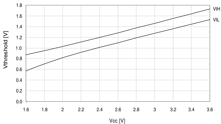
Figure 33-190. I/O pin input threshold voltage vs. V_{CC} .
