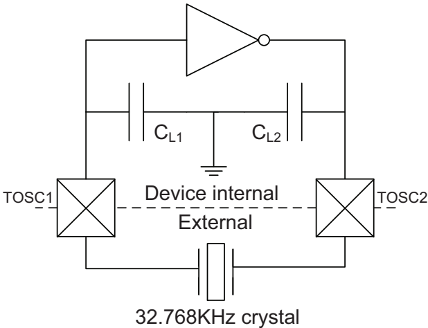
Figure 32-25.TOSC input capacitance.
