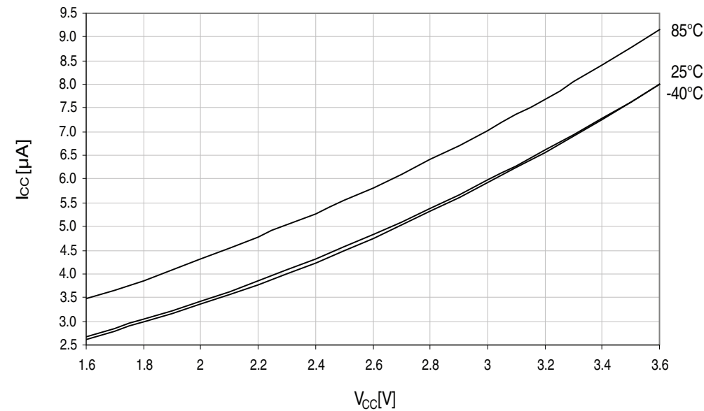
Figure 33-259. Standby supply current vs. V_{CC} . Standby, f_{SYS} = 1MHz .
