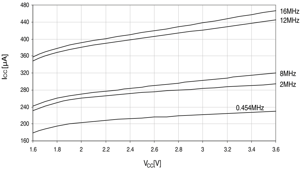
Figure 33-260. Standby supply current vs. V_{CC} . 25°C, running from different crystal oscillators.
