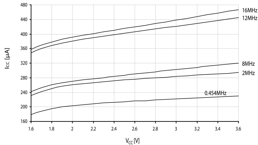
Figure 33-178. Standby supply current vs. V_{CC} . 25°C, running from different crystal oscillators.
