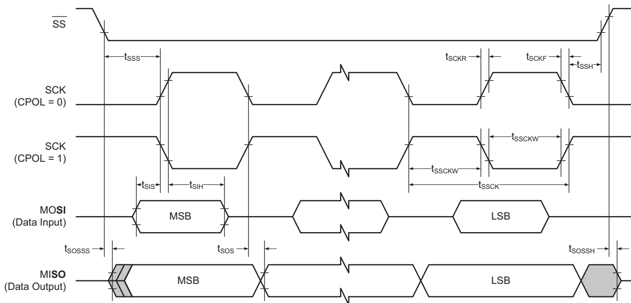
Figure 32-13. SPI timing requirements in slave mode.
