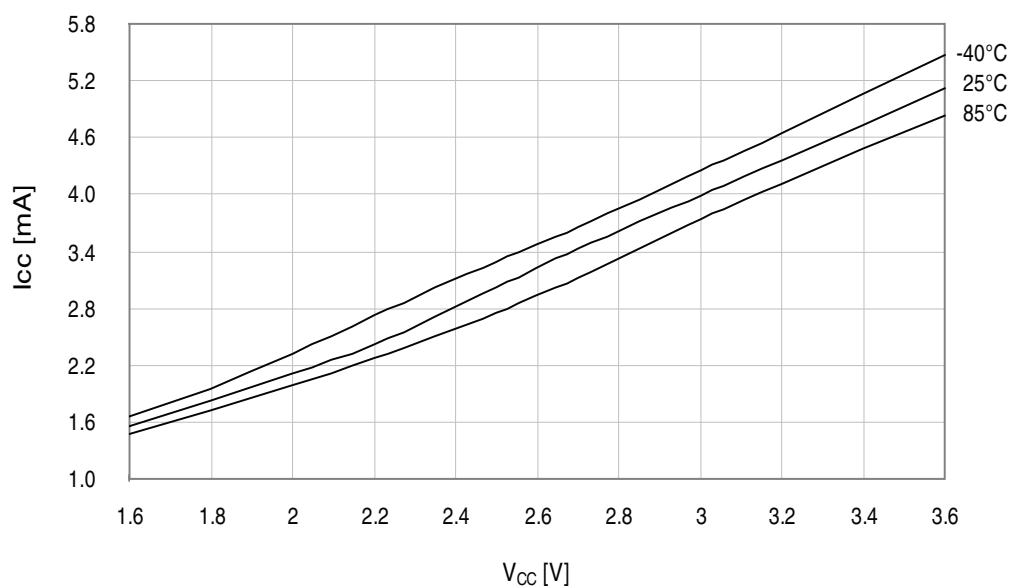
Figure 33-246. Active mode supply current vs. V_{CC} .
