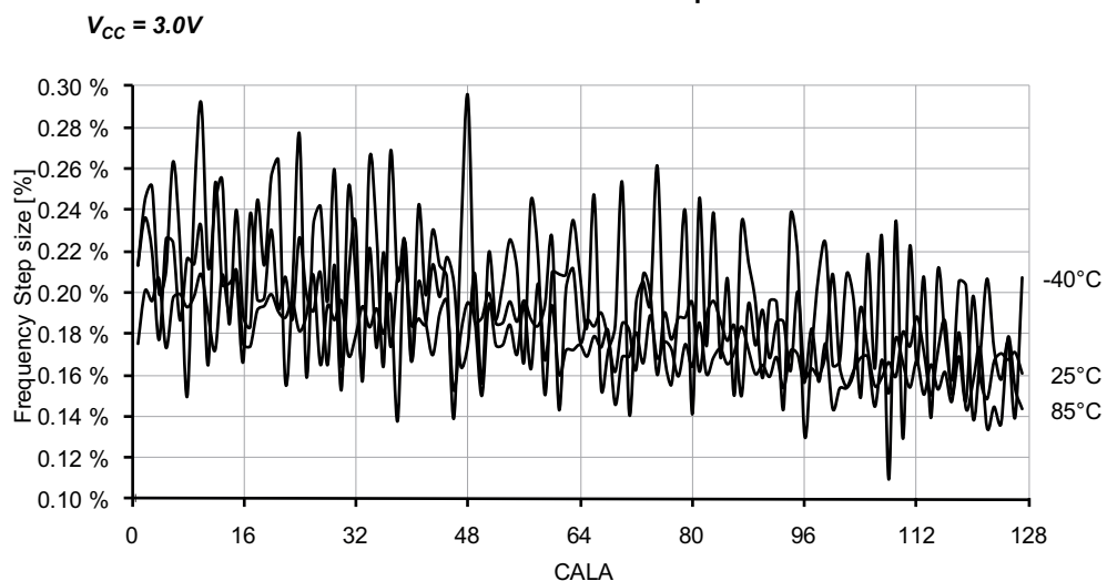
Figure 33-237. 48MHz internal oscillator CALA calibration step size.
