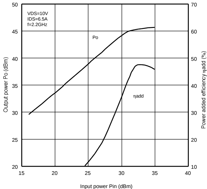
Po, \eta_{add} vs. Pin
