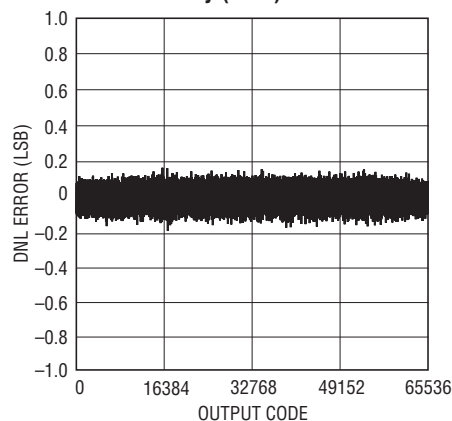
LTC2161: Differential Non-Linearity (DNL)
