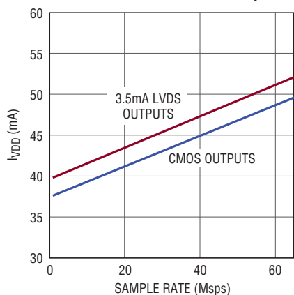
LTC2162: I_{VDD} vs Sample Rate, 5MHz, -1dBFS Sine Wave Input
