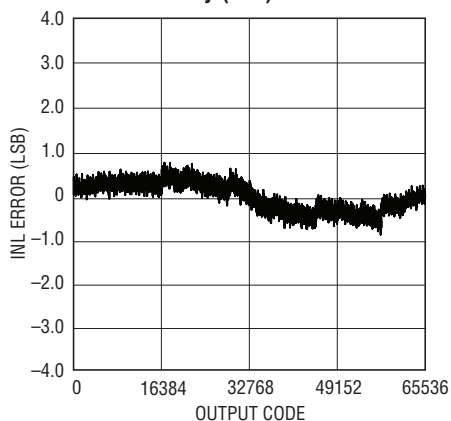
LTC2161: Integral Non-Linearity (INL)
