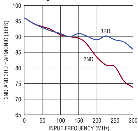
LTC2162: 2nd, 3rd Harmonic vs Input Frequency, -1dBFS, 65Mps, 1V Range
