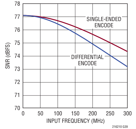
LTC2160: SNR vs Input Frequency, -1\text{dBFS} , 25\text{Mpsps} , 2\text{V} Range
