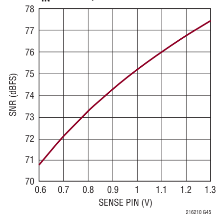
LTC2160: SNR vs SENSE, f_{IN} = 5\text{MHz} , -1\text{dBFS}
