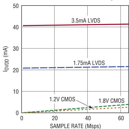
LTC2162: I_{OVPD} vs Sample Rate, 5MHz, -1dBFS Sine Wave Input
