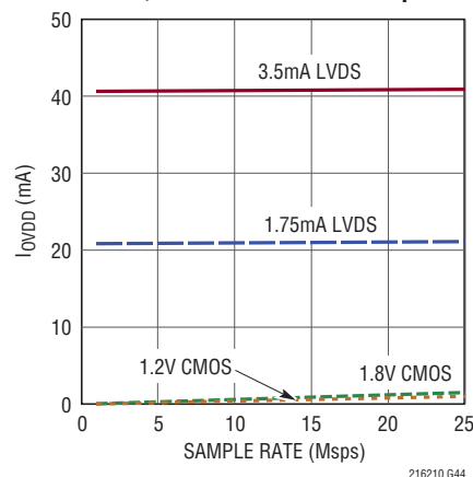
LTC2160: I_{OVD} vs Sample Rate, 5\text{MHz} , -1\text{dBFS} Sine Wave Input
