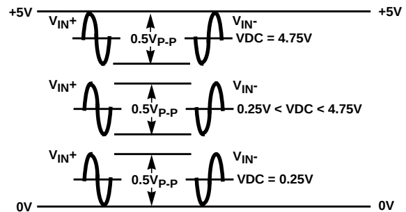
FIGURE 4. DIFFERENTIAL ANALOG INPUT COMMON MODE VOLTAGE RANGE
