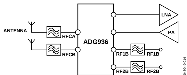
Figure 28. Tx/Rx Switching
