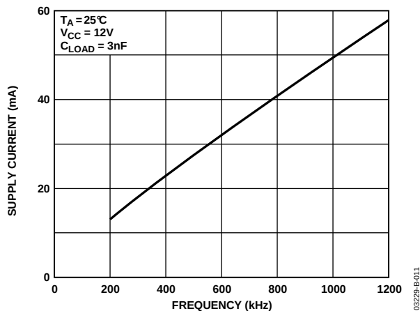
Figure 11. Supply Current vs. Frequency
