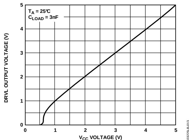
Figure 13. DRVL Output Voltage vs. Supply Voltage
