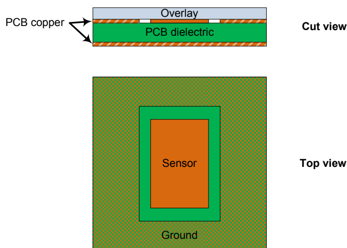
Figure 26 – Typical Capacitive Sensing Implementation
