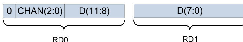
Figure 54 – Channel Data Format
