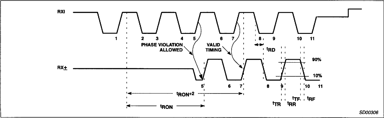
Figure 4. Receiver Timing
