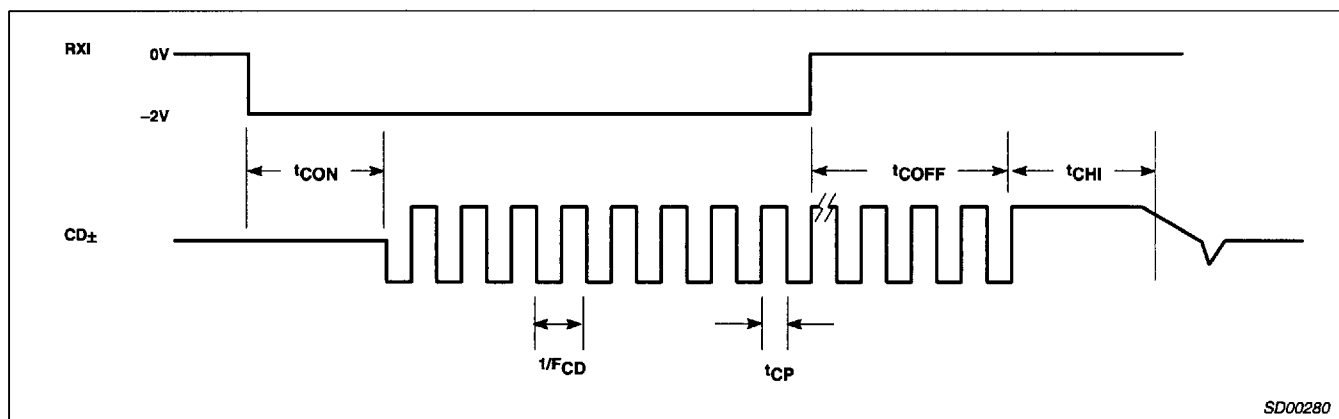
Figure 7. Collision Timing
