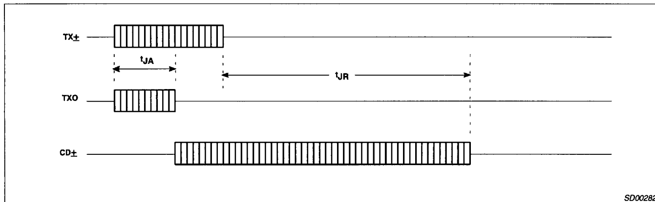
Figure 9. Jabber Timing
