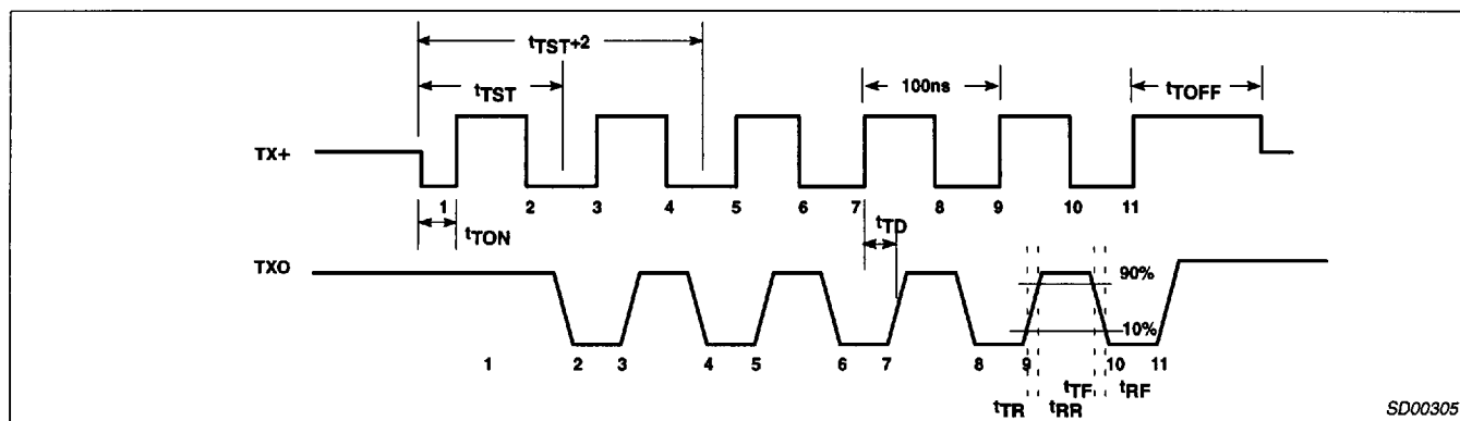
Figure 6. Transmitter Timing
