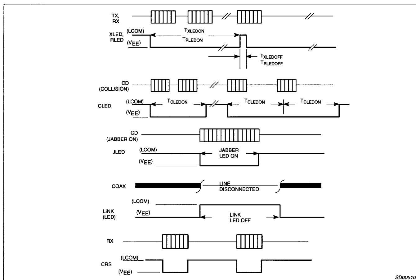
Figure 10. LED Timing
