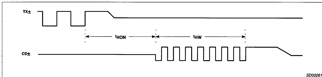
Figure 8. Heartbeat Timing
